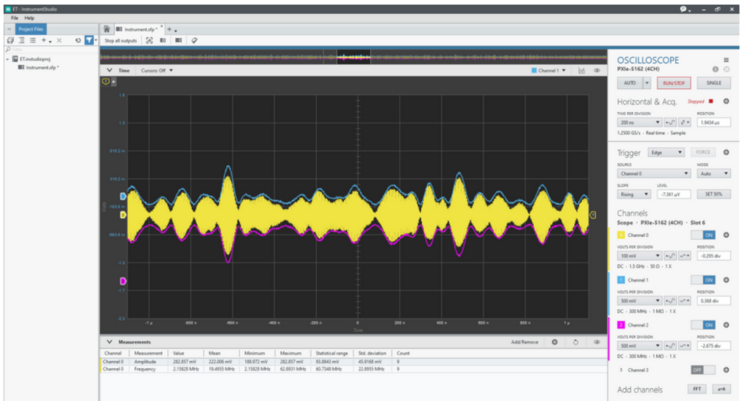
FIGURE 4 Using RFmx to Perform Envelope Tracking and Multi-Instrument Synchronization
