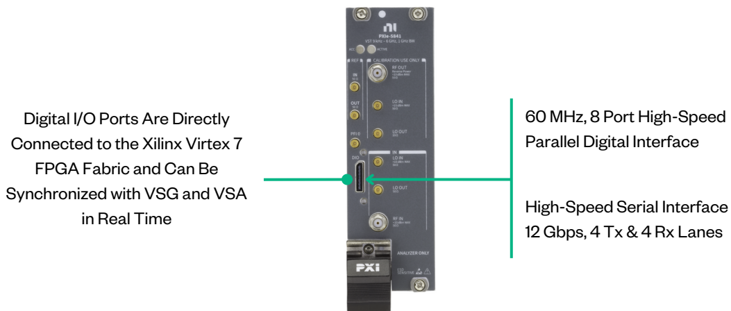
Digital Interfacing Ports on the PXle-5841 Front Panel
