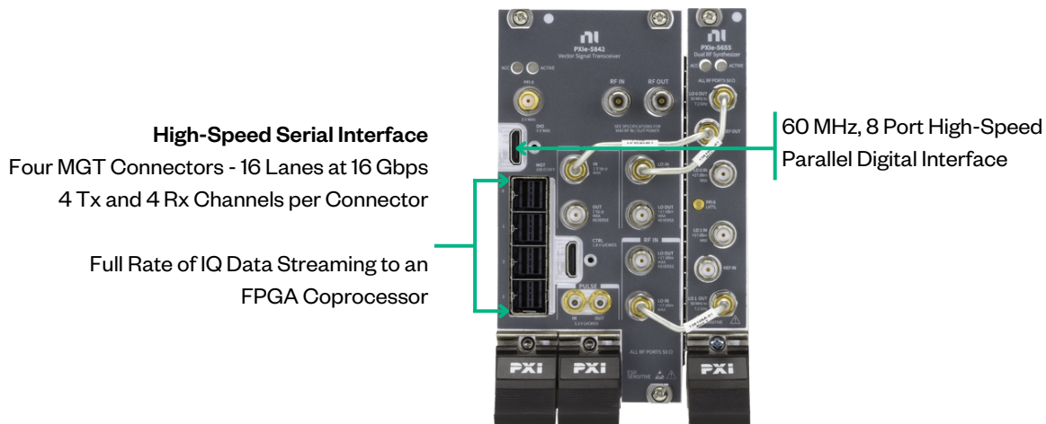
Digital Interfacing Ports on the PXle-5842 Front Panel
