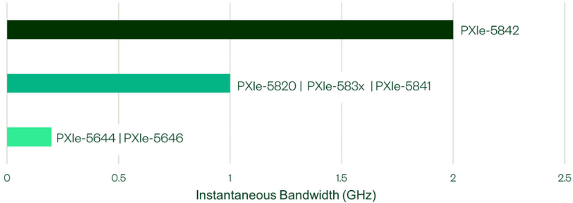
FIGURE 2 Instantaneous RF Bandwidth in GHz of NI VST Models
